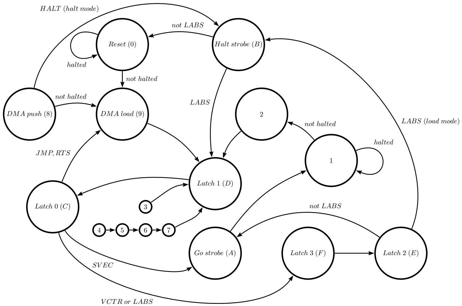
Figure 1: State transition diagram for the Atari DVG
